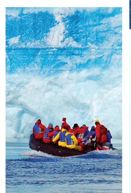
Ice wall, Paradise harbour, Antarctica
